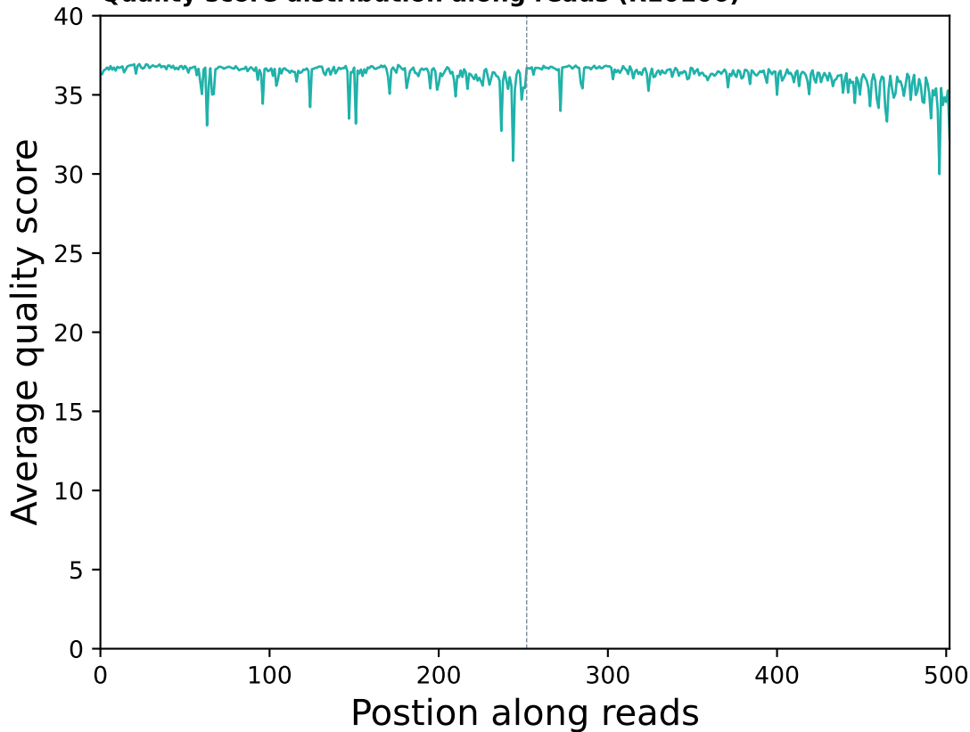
Quality score distribution along reads (R10106)
